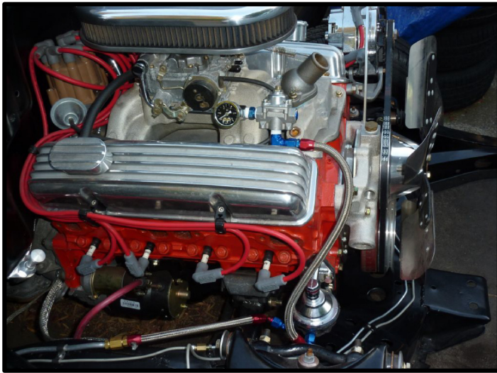
The fuel lines have been connected to the engine mounted fuel pump and to the carburetor through a pressure regulator.
