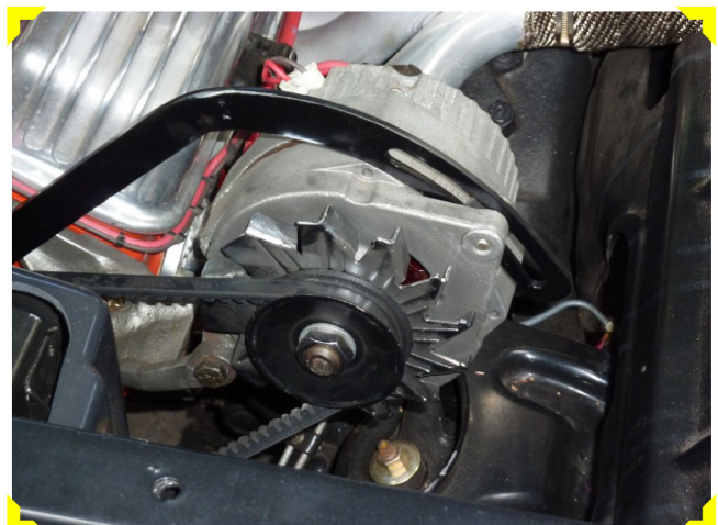
I had to weld two different brackets together to obtain enough length and bend on the replacement bracket.
